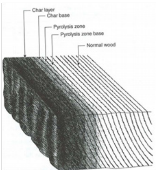
Figure 3.1. Formation of Char layer and pyrolysis zone in wood (one-dimensional) when exposed to high temperatures (CSA, 2011).
